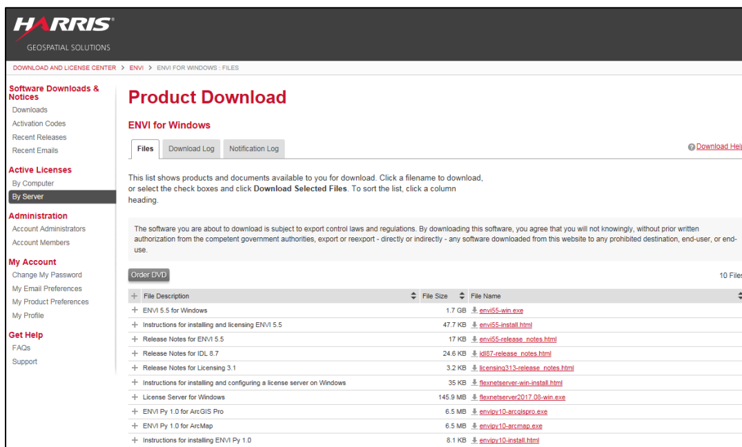
図 6 : Product Download
